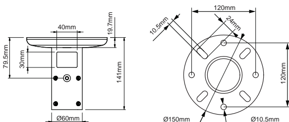
CEILING MOUNT
