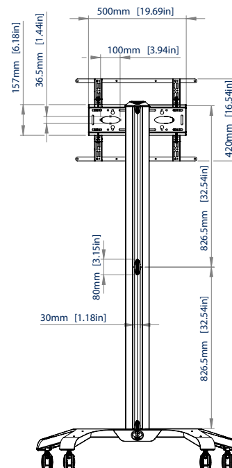
REAR VIEW
