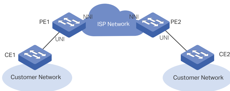
Figure 1-1 L2PT Application
