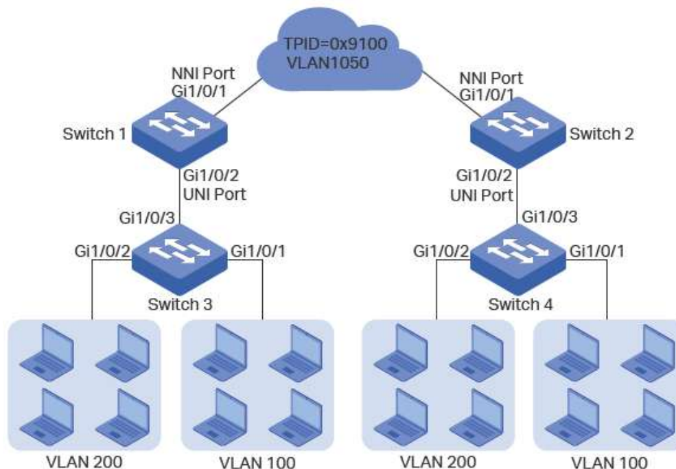
Figure 4-1 Network Topology
