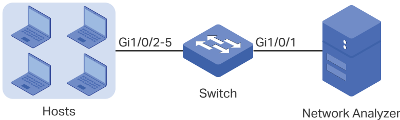
Figure 2-1 Network Topology
