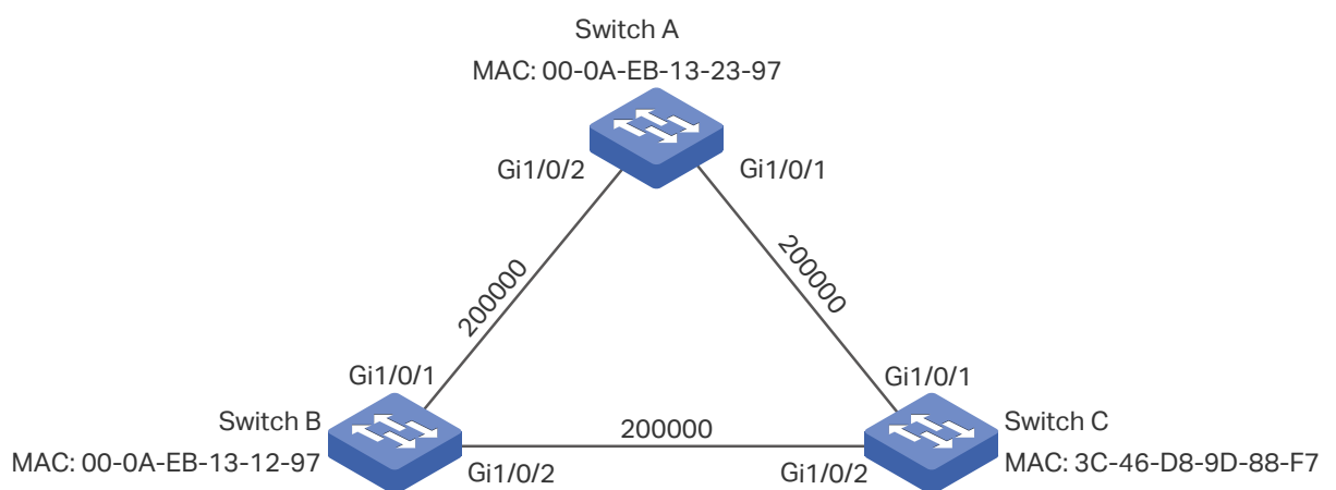
Figure 5-1 Network Topology
