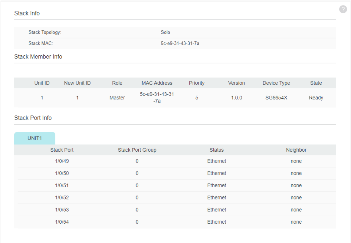
Figure 5-1 Stack Info
